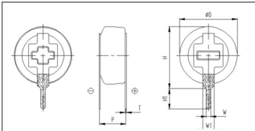
PIN TYPE B
