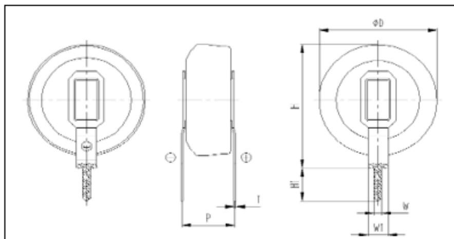
PIN TYPE A
